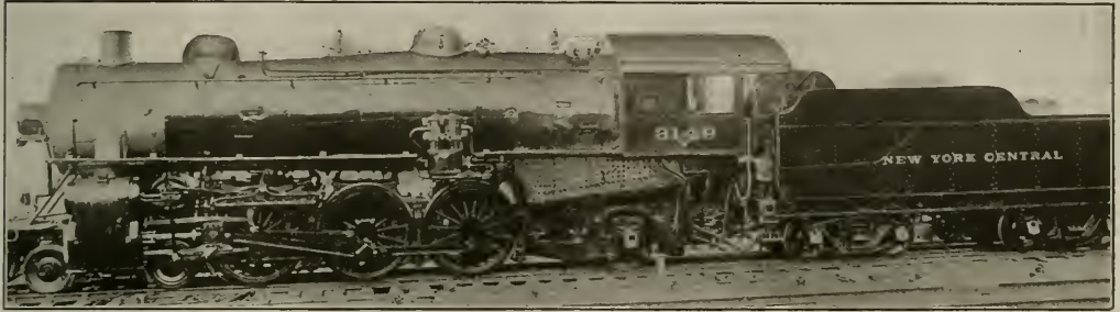
PACIFIC TYPE LOCOMOTIVE EQUIPPED WITH LOCOMOTIVE BOOSTER NEW YORK CENTRAL RAILROAD
